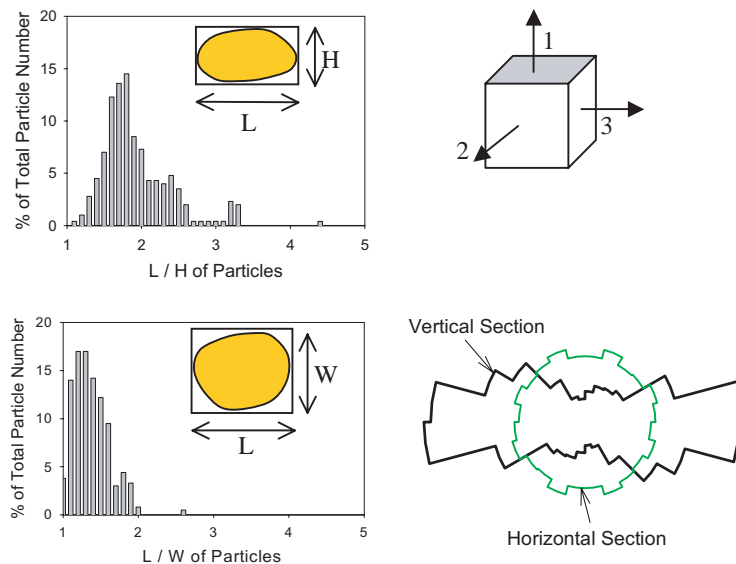
Fig. 10. Distributions for grain shape and grain orientation.
