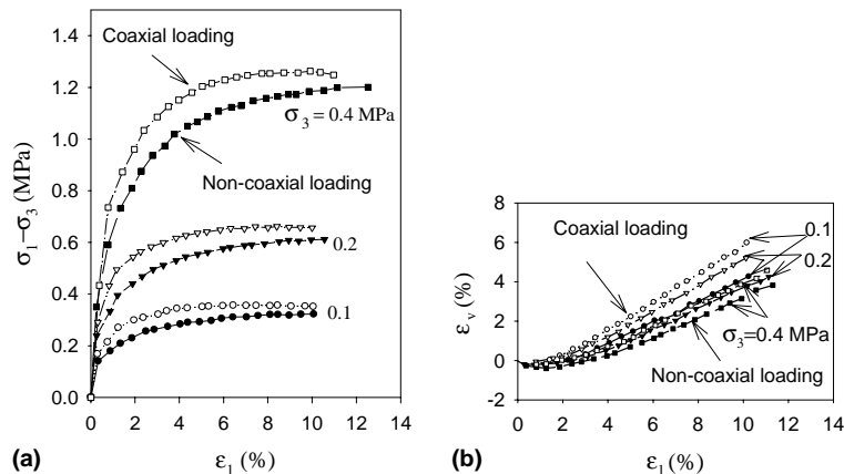
Fig. 12. Cubical triaxial experimental results: (a) stress–strain curves, and (b) volumetric strain vs. axial strain curves.
